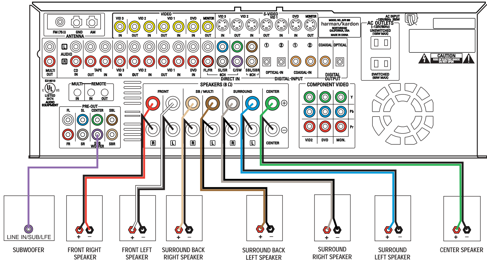
Figure 2 – Speaker Connections
